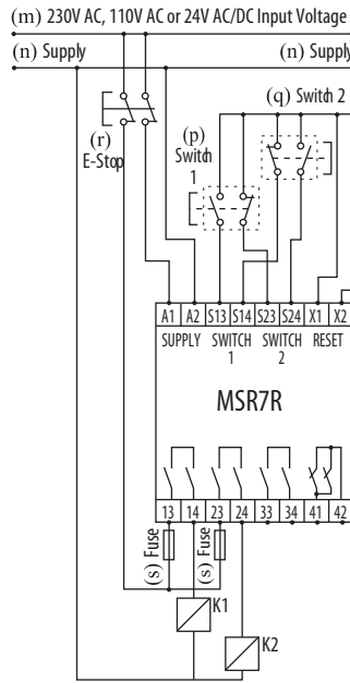
(u) 2 Hand controller with E-Stop.
