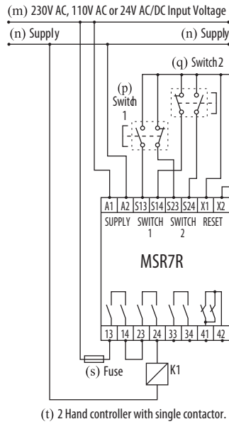
(t) 2 Hand controller with single contactor.
