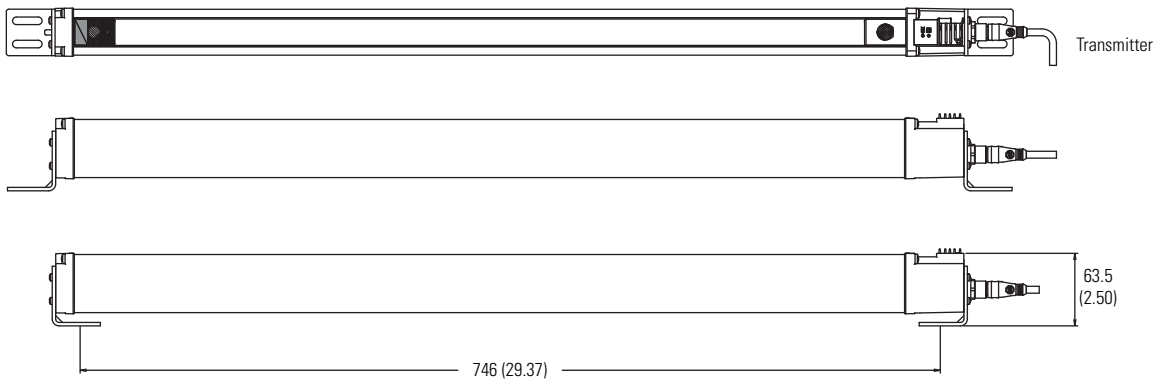
440L-P4A2500YD consists of a pair 440L-T4A2500YD transmitter & 440L-R4A2500YD receiver
