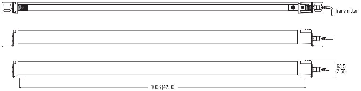
440L-P4A3400YD consists of a pair 440L-T4A3400YD transmitter & 440L-R4A3400YD receiver
