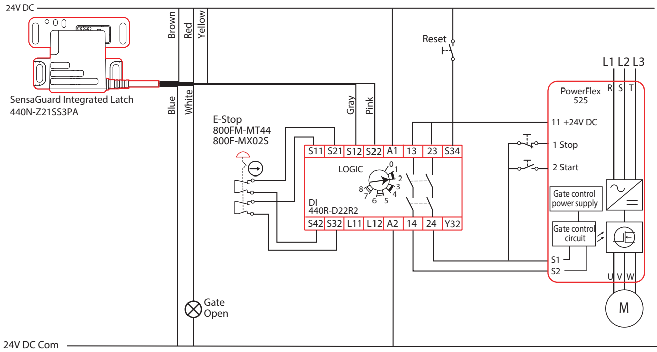
Figure 19 - DI Safety Relay with SensaGuard Integrated Latch and PowerFlex 525 Drive
