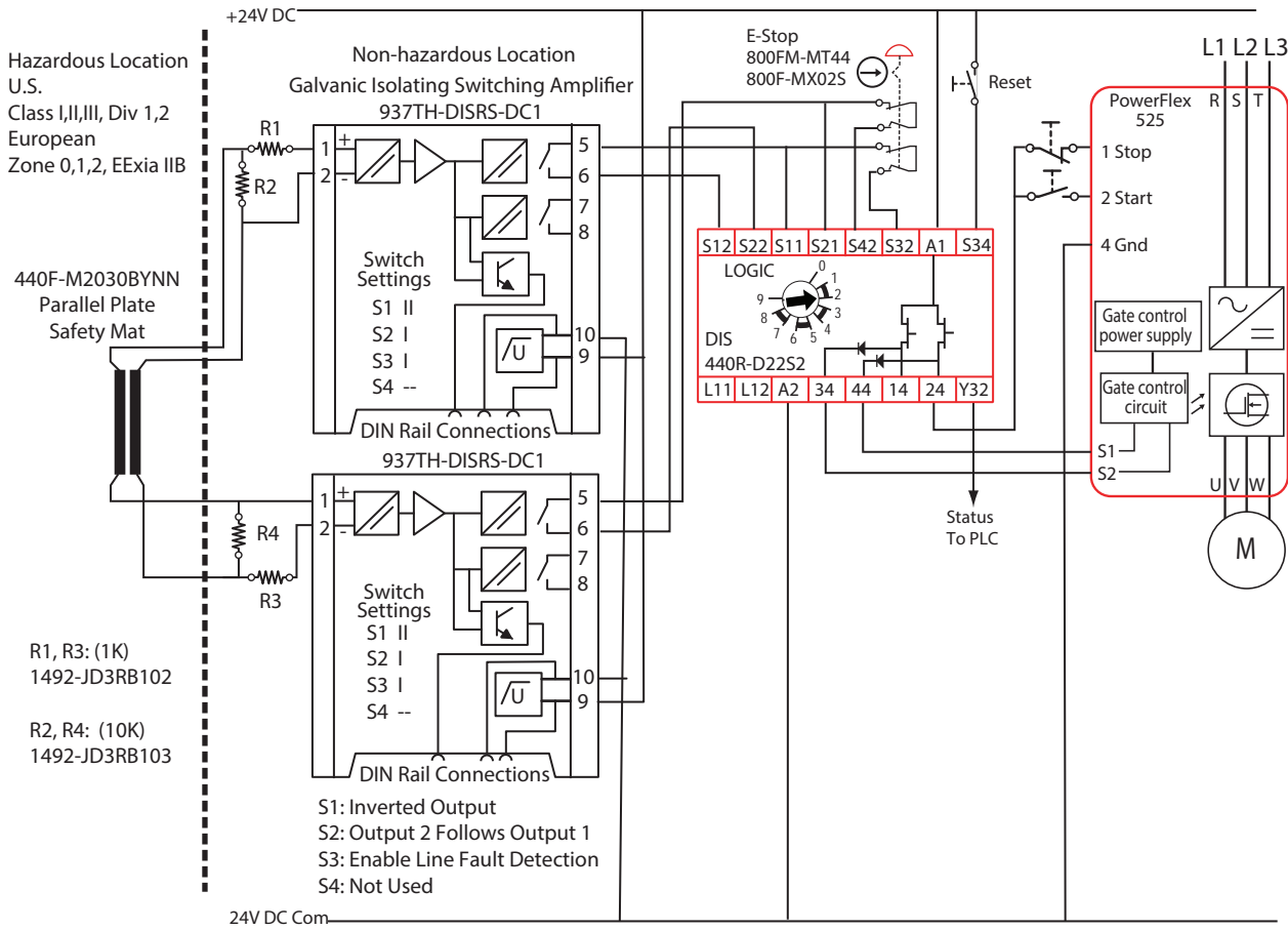
Figure 30 - Hazardous Location
