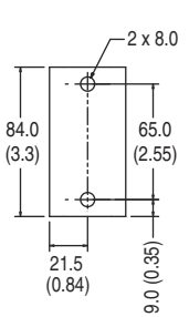
440J-A04N Double Safety Switch Bracket
