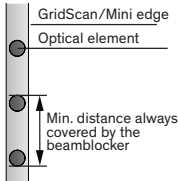
Figure 9: Door blanking
