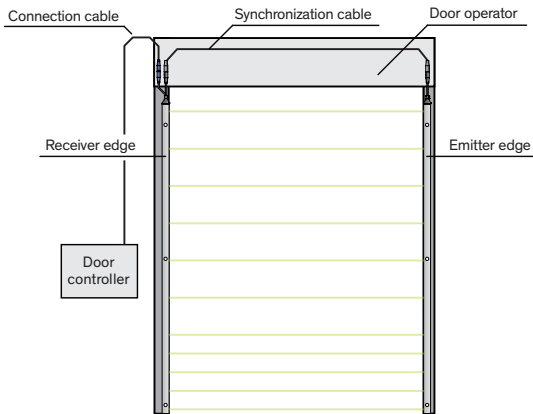
Figure 6: GridScan/Mini-SB2/-ST2 application (overview)
